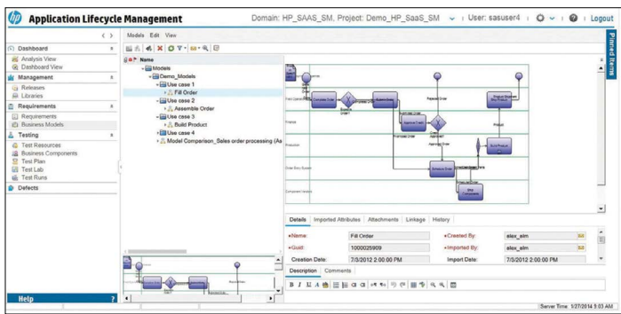
Figure 3. Importing a business process model in ALM and aligning business process to requirements.
