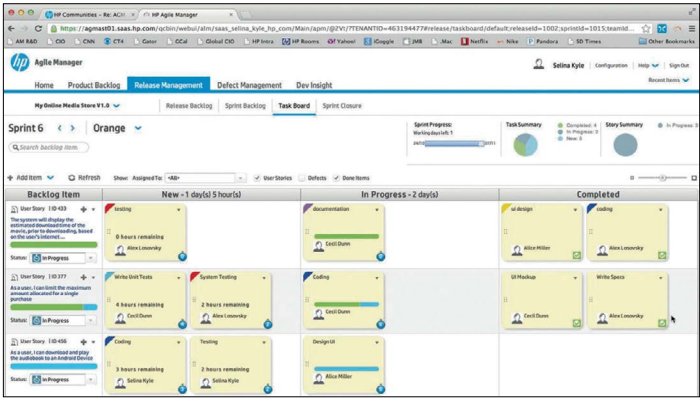
Figure 4. Agile Manager task board interface.
