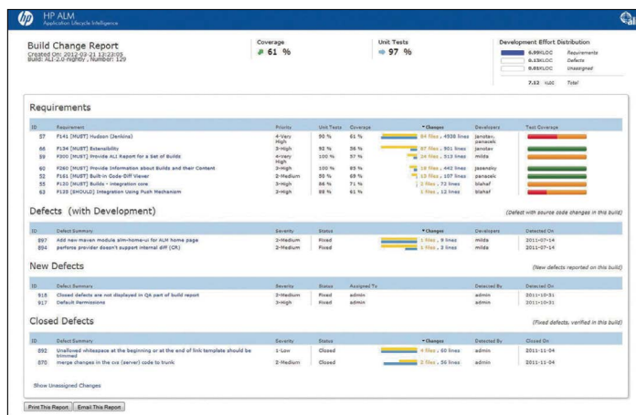
Figure 2. ALI builds changes report and increases agility with continuous delivery best practices.
