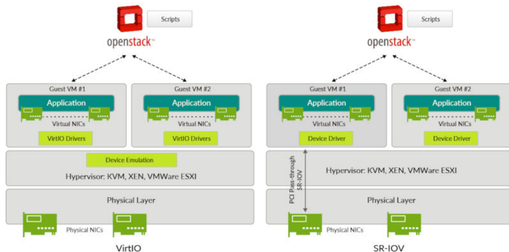
Figure 1: The vMX architecture for VirtIO and SR-IOV.
