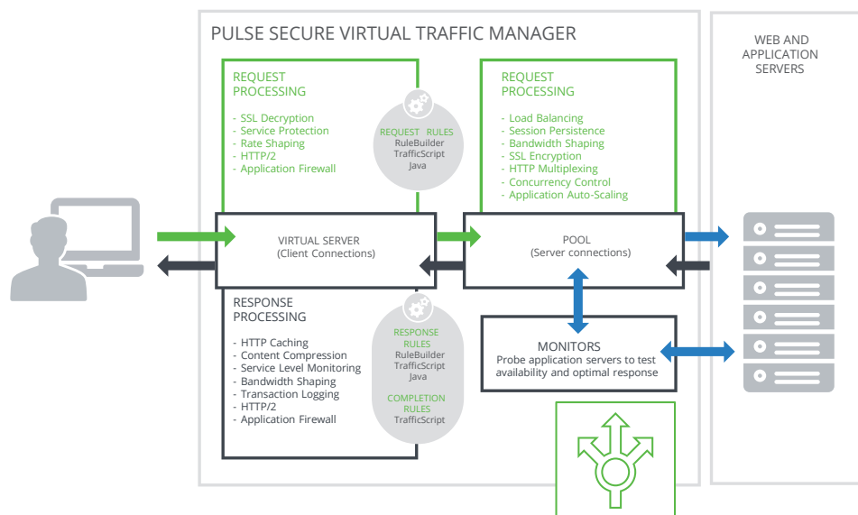
Figure 1. The advanced capabilities in the Pulse Secure Virtual Traffic Manager can be enhanced using TrafficScript or Java extensions.
